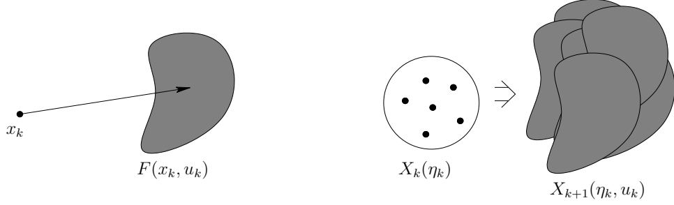
Figure 29: The first step in computing the nondeterministic I-state is to take the union of F(x_k, u_k) over all possible x_k \in X_k(\eta_k) . It is the effect of applying an action when the current state is not precisely known.
