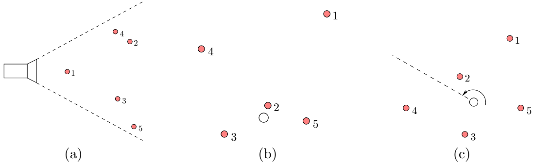
Figure 16: Three kinds of compound relational sensors: (a) The linear sensor observes that the landmarks are ordered from left to right as (4, 2, 1, 3, 5). (b) This sensor sorts the landmarks closest to farthest, resulting in the observation (2, 3, 5, 4, 1). (c) The cyclic sensor sweeps counterclockwise and yields the cyclic ordering (1, 2, 4, 3, 5)
