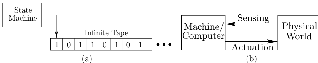
Figure 1: (a) For classical computation, the full state is given by the finite machine state, the head position, and the binary string written on the tape. (b) In this paper, there is both an internal computational state and an external physical state.
