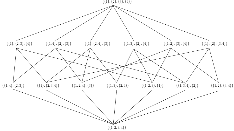
Figure 20: The partition lattice for a four-element set. The best and worst sensors are at the top and bottom, respectively.
