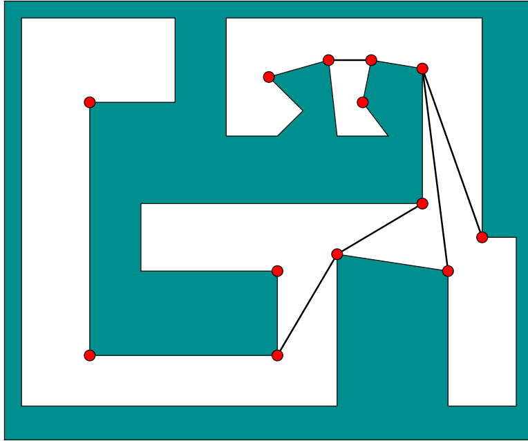
Figure 38: The shortest-path graph. It is sometimes referred to as a (reduced) visibility graph [34].
