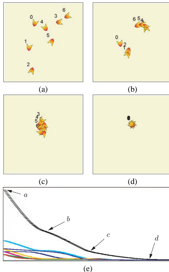
Fig. 1. Screen captures from simulation program. a) - d) Four snapshots of a seven-agent rendezvous, one running after the other. e) Plot of the Lyapunov function of the rendezvous, with a-d on the plot corresponding to the four snapshots.
