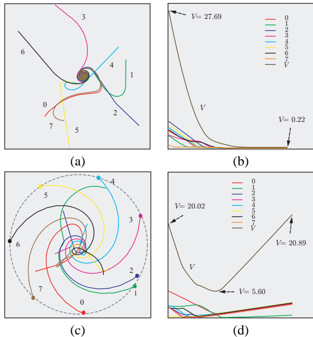
Fig. 5. a) Eight-agent cyclic pursuit, which converges, with \phi = 0.35 , \omega = 2.0 , and \Delta t = 0.1s . b) Plot of the Lyapunov function for (a), with numbered lines being individual \ell_{i,i+1} terms. c) Diverging case with \phi changed to 0.6 holding other conditions the same. The agents arrange themselves on a cycle quickly as they spin away from each other. Dots are the agents' positions as of the last snapshot. d) Plot of the Lyapunov function for (c).
