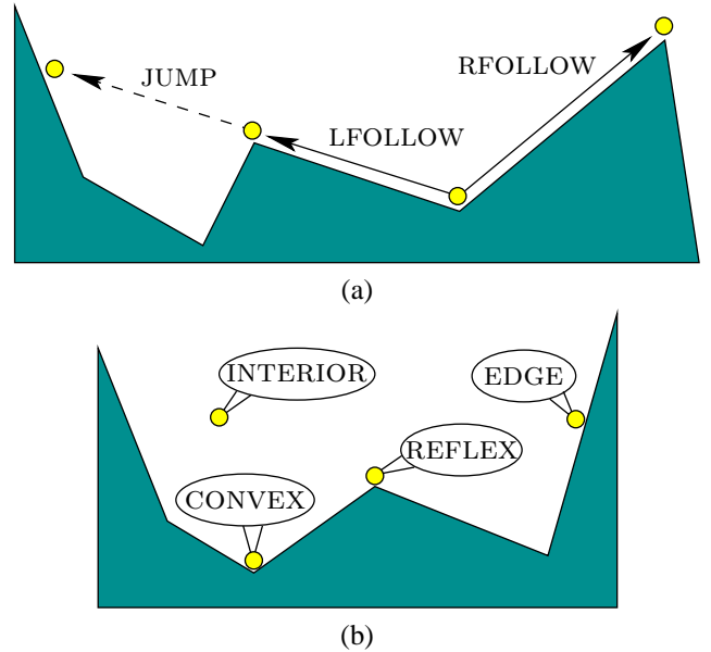
Fig. 1. (a) The robot can execute three movements: following the wall when it is to the right (RFOLLOW), following it on the left (LFOLLOW), and jumping straight to the next wall, traveling past a reflex vertex (JUMP). (b) The robot has a sensor that can distinguish between being in the interior, at a convex vertex, at a reflex vertex, or in the interior of an edge.
