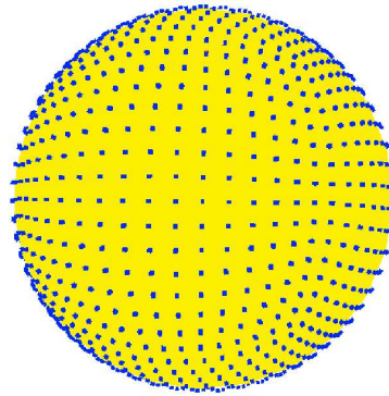
Fig. 1. Distribution of points on the sphere S^2 generated by a grid (Sukharev [20]) on each spherical face.
