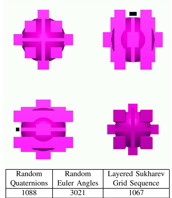
Fig. 2. This problem involves moving a robot (black) from the north pole to the south pole. Multiple views of the geometry of the problem are shown (obstacles are drawn in lighter shades) as well as comparisons of the number of nodes generated by different sampling strategies.
